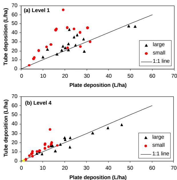
Figure 10. Effects of droplet size on deposition on paired plate and tube collectors (a) at the top of the canopy and (b) at the bottom of the canopy.
