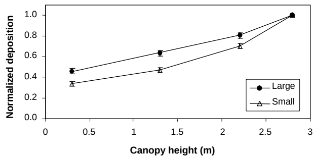
Figure 11. Attenuation of normalized mean spray deposition on tubes versus height above the ground.
