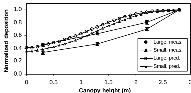
Figure 13. Comparison of measured and modeled spray attenuation through a radiata pine canopy using large and small droplets. The canopy model is based on LAI-2000 measurements.
