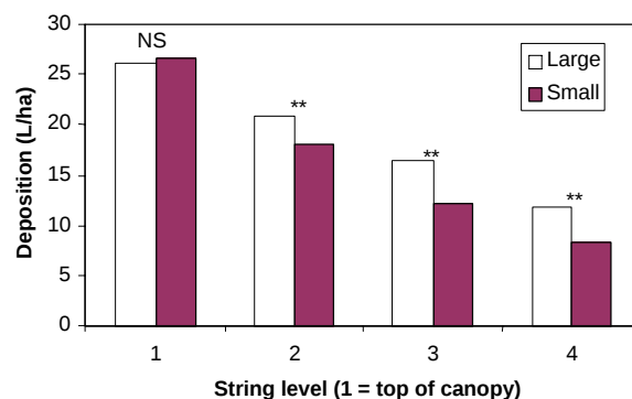
Figure 9. Effect of droplet size and sample height on adjusted spray deposition on tubes. (** = significant difference between droplet sizes ( p = 0.01 )).
