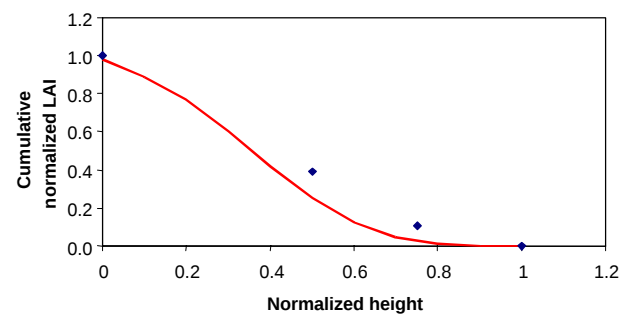
Figure 7. Cumulative normalized leaf and foliage area indices, based on destructive sampling and LAI-2000 measurements, respectively, plotted against normalized canopy height.
