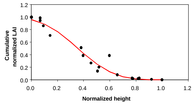
Figure 6. Cumulative normalized leaf area index (plot level) versus normalized height with a modified Weibull function (solid line) fitted to measurements (points).
