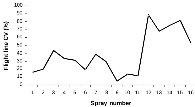
Figure 5. Average coefficient of variation (CV) for flight line spacing for each spray application.
