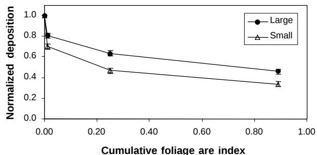
Figure 12. Attenuation of normalized mean spray deposition on tubes versus cumulative projected foliage area, summed from the top of the canopy down.
