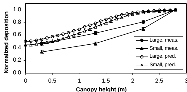
Figure 14. Comparison of measured and modeled spray attenuation through a radiata pine canopy using large and small droplets. The canopy model is based on measured leaf area.
