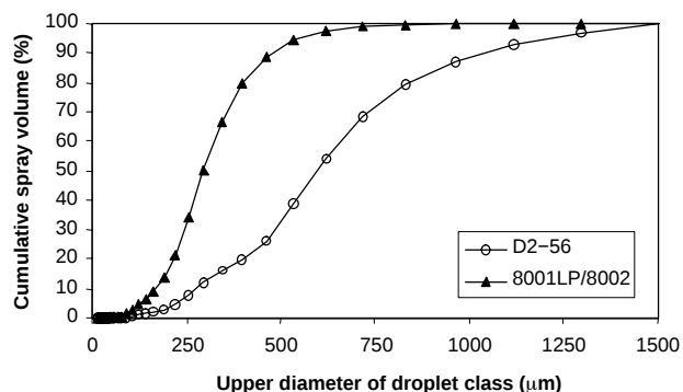
Figure 4. Percentage total spray volume contained within droplets of a size equal to or less than any specified diameter.
