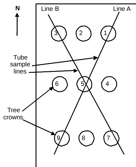
Figure 2. Inner sample plot layout.
